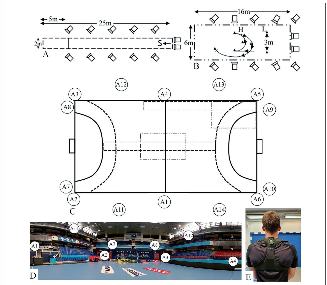
FIG. 1. A: Position of the Vicon camera on configuration for sprints (---); B: Position of the Vicon camera on configuration for lateral and specific movements (....); C: Schematic position of the Kinexon antennas and position of testing zones on the field; D: Position of Kinexon antennas; E: Position of the Vicon reflective marker on the Kinexon tag
